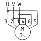
HOIST MOTOR CIRCUIT DIAGRAM OF 220,230V
