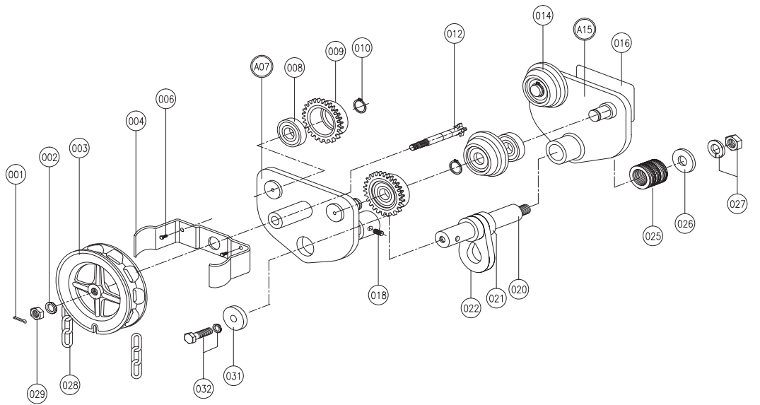
10TON GEAR TROLLEY
