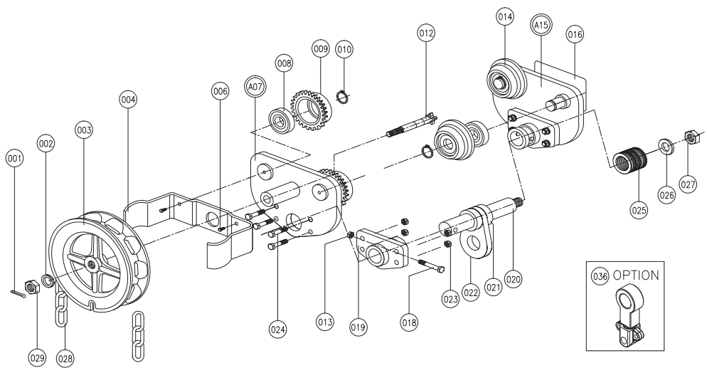
1/2~5TON GEAR TROLLEY
