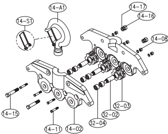
14-00 TOP HOOK ASS'Y
