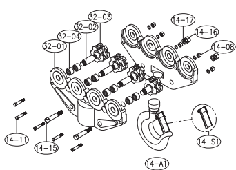
32-00 BOTTOM HOOK ASS'Y
