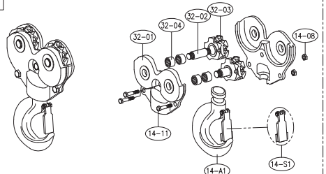
32-00 BOTTOM HOOK ASS'Y
