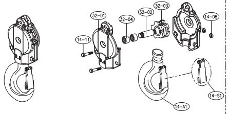
32-00 BOTTOM HOOK ASS'Y
