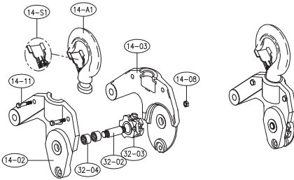
14-00 TOP HOOK ASS'Y
